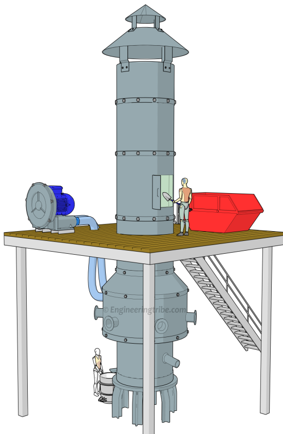
Cupola Furnace
